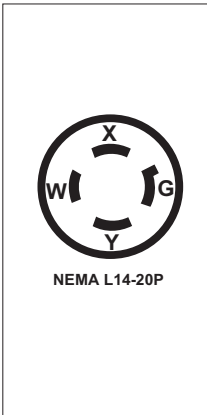
L14-20 SINGLE 20A - 125/250 Volt Twist Lock 4 - WIRE (optional) #13
