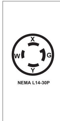
L14-30 SINGLE 30A - 125/250 Volt Twist Lock 4 - WIRE (optional) #15
